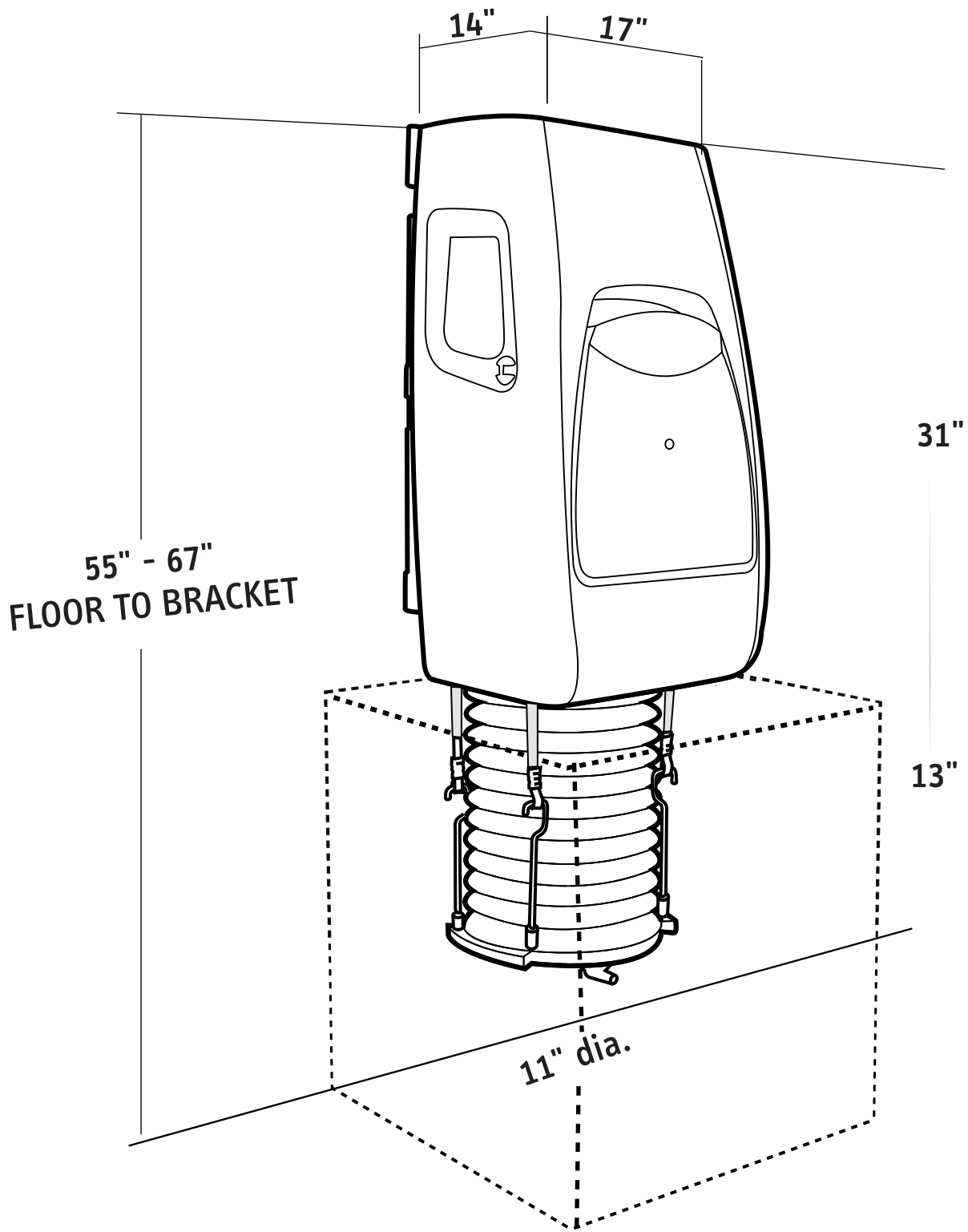
Fendall 2000 Emergency eyewash Overall Dimensions
