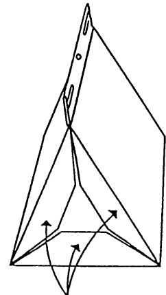
End panels should slope inward
